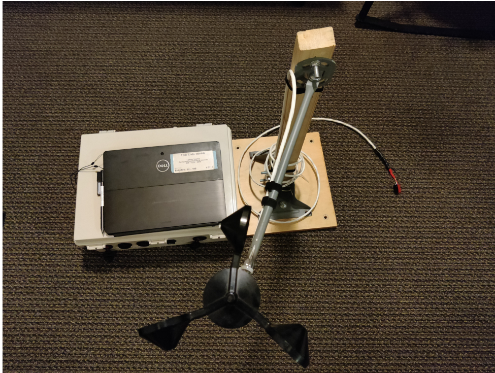
Fig.1 Current Analysis & Wind Turbine Subsystem
